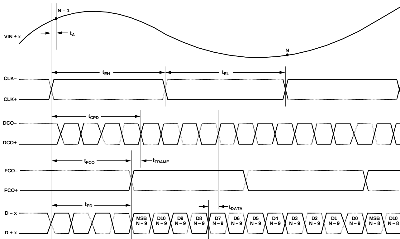
Figure 2. 12-Bit Data Serial Stream, MSB First (Default)
