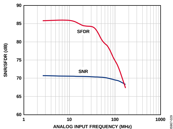
Figure 39. SNR/SFDR vs. f_{IN} , AD9222-50
