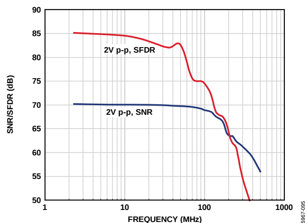
Figure 40. SNR/SFDR vs. f_{IN} , AD9222-65
