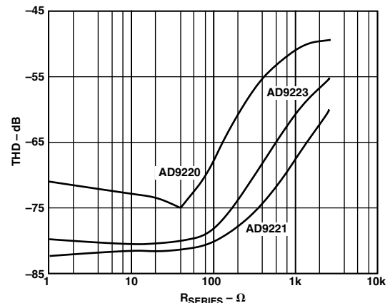
Figure 8. THD vs. R_{\text{SERIES}} ( f_{\text{IN}} = f_S/2 , A_{\text{IN}} = -0.5 dB, Input Span = 2 V p-p, V_{\text{CM}} = 2.5 V)
