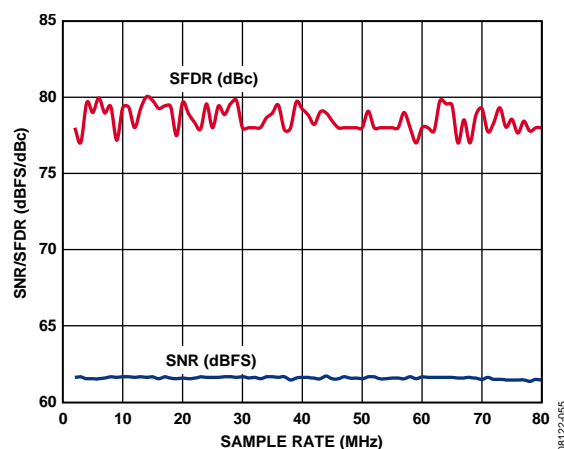
Figure 13. AD9204-80 SNR/SFDR vs. Sample Rate with f_{IN} = 9.7 MHz
