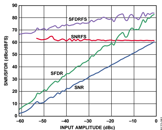
Figure 15. AD9204-80 SNR/SFDR vs. Input Amplitude (AIN) with f_{IN} = 9.7 MHz
