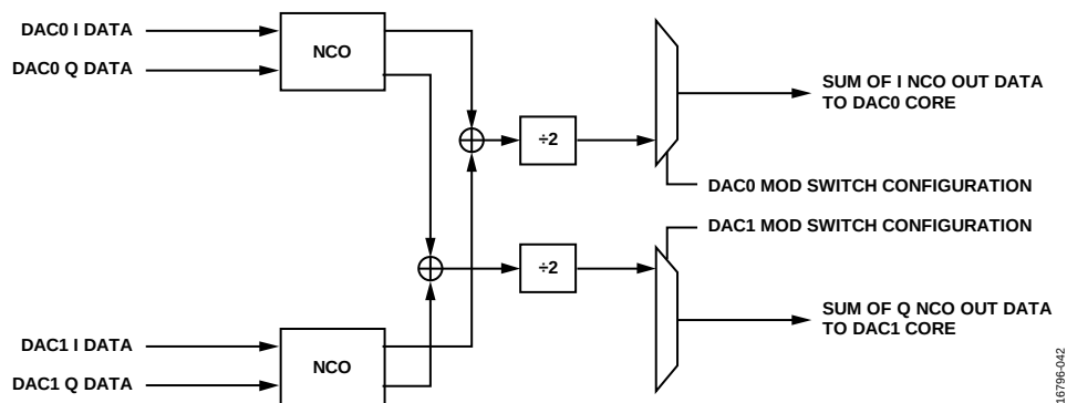
Figure 82. Configuration 1, CMPLX_MOD_DIV2_DISABLE = 0—DAC0 = I0 + I1, DAC1 = Q0 + Q1
