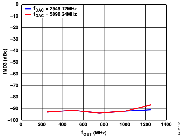
Figure 23. IMD3 vs. f_{OUT} over f_{DAC} (Mode 0), Channel Interpolation 2 \times , Main Interpolation 8 \times , 1 MHz Tone Spacing
