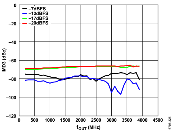
Figure 29. IMD3 vs. f_{OUT} over Digital Scale (Mode 12), 8 GHz DAC Sampling Rate, Channel Interpolation 1x, Main Interpolation 2x, 1 MHz Tone Spacing
