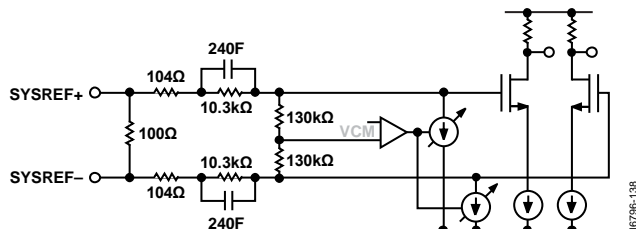
Figure 61. DC-Coupled SYSREF± Receiver Circuitry
