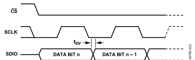
Figure 52. Timing Diagram for Serial Port Register Read
