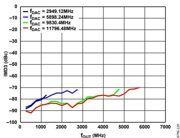
Figure 23. IMD3 vs. f_{OUT} over f_{DAC} (Mode 1), Channel Interpolation 4 \times , Main Interpolation 8 \times , 1 MHz Tone Spacing, -7 dB Digital Scale
