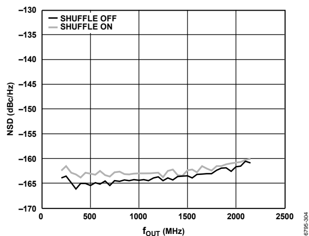
Figure 32. NSD vs f_{OUT} , 11796.48 MHz f_{DAC} , 12-Bit Resolution for Different Shuffle Options, Single-Tone, Measured at 70 MHz
