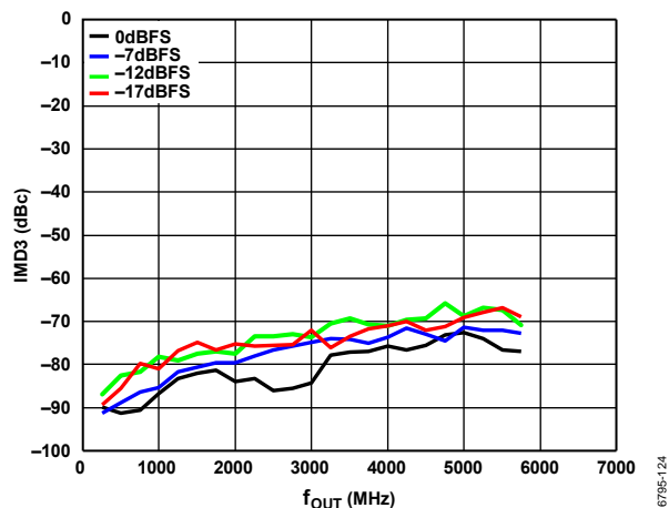
Figure 27. IMD3 vs. f_{OUT} over Digital Scale (Mode 9), 12 GHz DAC Sample Rate, Channel Interpolation 1 \times , Main Interpolation 12 \times , 1 MHz Tone Spacing
