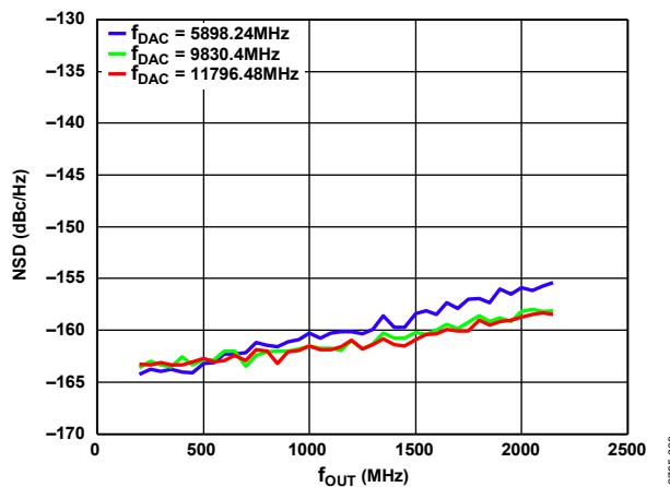
Figure 31. NSD vs. f_{OUT} over f_{DAC} , 16-Bit Resolution, Shuffle On, Single-Tone, Measured at 10% Offset from f_{OUT}
