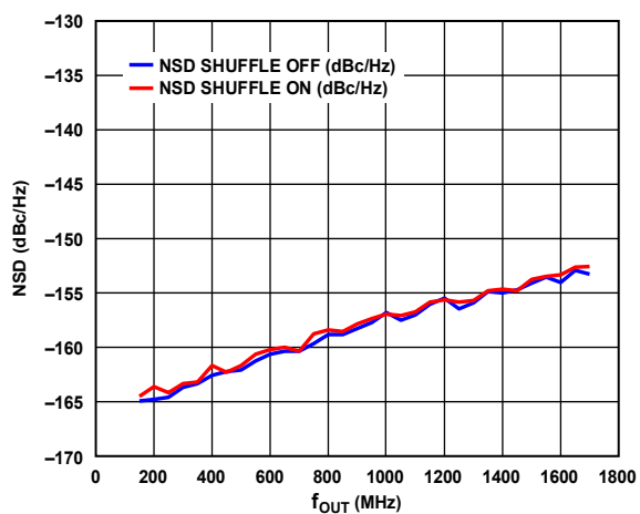
Figure 35. Single-Tone NSD Measured at 70 MHz vs. f_{OUT} , 3.4 GHz f_{DAC} , 11-Bit Resolution, Shuffle Off vs. Shuffle On
