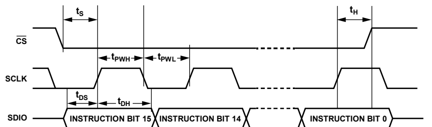
Figure 53. Timing Diagram for Serial Port Register Write
