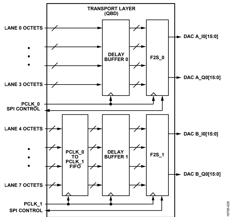
Figure 71. Transport Layer Block Diagram
