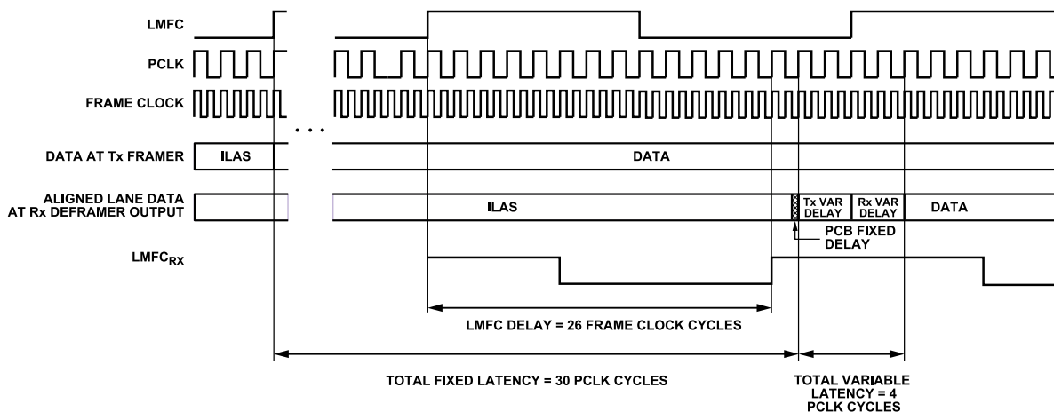
Figure 62. LMFC Delay Calculation Example
