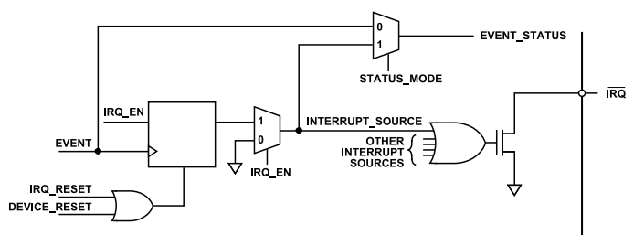
Figure 81. Simplified Schematic of \overline{\text{IRQx}} Circuitry
