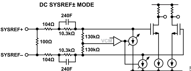
Figure 57. DC-Coupled SYSREF± Receiver Circuitry
