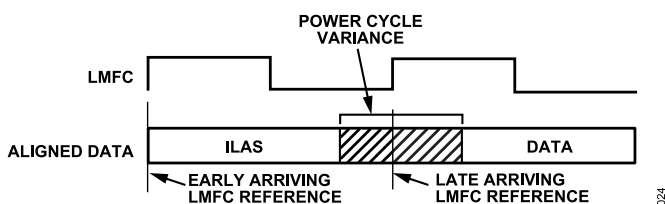
Figure 60. Link Delay &gt; LMFC Period Example
