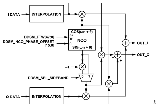
Figure 76. NCO Modulator Block Diagram
