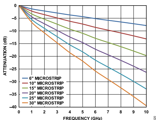
Figure 54. Insertion Loss of 50 Ω Microstrips on FR4
