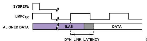
Figure 55. DYN_LINK_LATENCY Illustration
