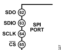
Figure 36. SPI Pins
