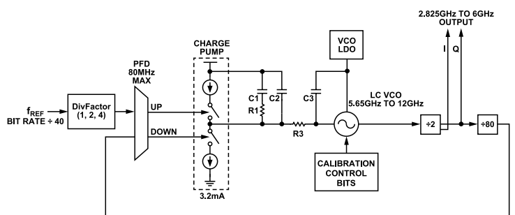
Figure 47. SERDES PLL Synthesizer Block Diagram Including VCO Divider Block
