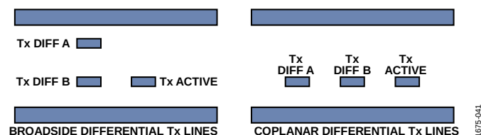
Figure 66. Broadside vs. Coplanar Differential Stripline Routing Techniques
