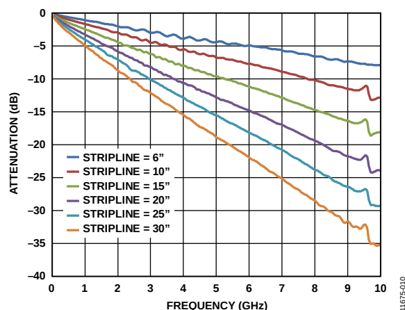
Figure 40. Insertion Loss of 50 \Omega Striplines on FR4
