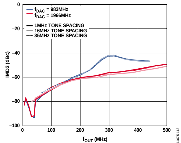
Figure 13. Two-Tone Third IMD (IMD3) vs. f_{OUT} over Tone Spacing at 0 \text{ dB Back Off} , f_{DAC} = 983 \text{ MHz} and 1966 \text{ MHz}
