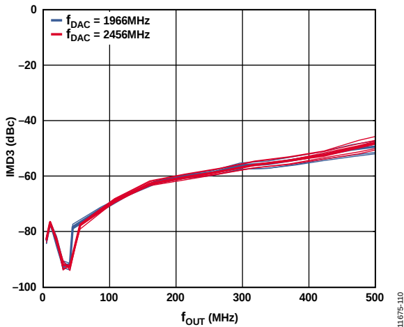
Figure 10. Two-Tone Third IMD (IMD3) vs. f_{OUT} , f_{DAC} = 1966 \text{ MHz} and 2456 \text{ MHz}
