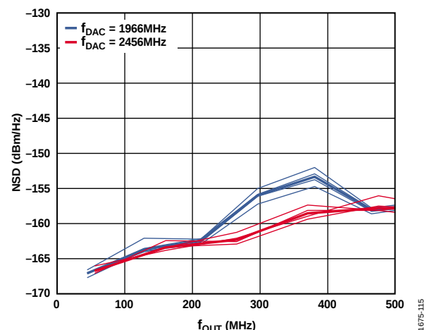
Figure 15. Single-Tone ( 0 \text{ dBFS} ) NSD vs. f_{OUT} , f_{DAC} = 1966 \text{ MHz} and 2456 \text{ MHz}
