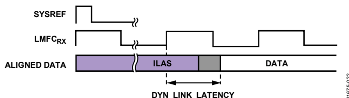
Figure 50. DYN_LINK_LATENCY Illustration
