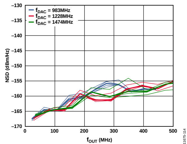
Figure 14. Single-Tone ( 0 \text{ dBFS} ) NSD vs. f_{OUT} , f_{DAC} = 983 \text{ MHz} , 1228 \text{ MHz} , and 1474 \text{ MHz}
