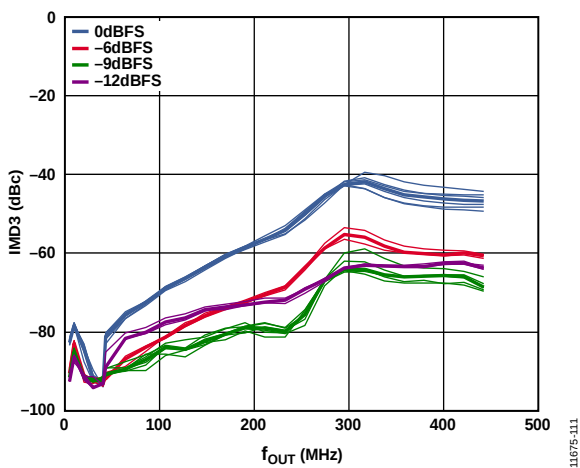
Figure 11. Two-Tone Third IMD (IMD3) vs. f_{OUT} over Digital Back Off, f_{DAC} = 983 \text{ MHz} , Each Tone Is at -6 \text{ dBFS}
