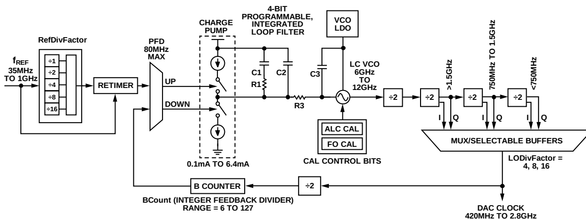
Figure 79. Device Clock PLL Block Diagram
