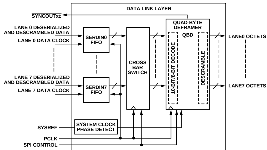
Figure 43. Data Link Layer Block Diagram
