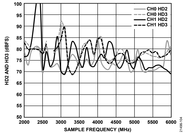
Figure 70. HD2 and HD3 vs. Sample Frequency ( f_s ), f_{IN} = 450 MHz, A_{IN} = -1 dBFS, f_s = 2 GSPS to 6 GSPS
