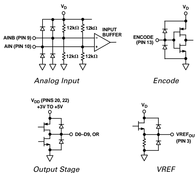
Figure 2. Equivalent Circuits
