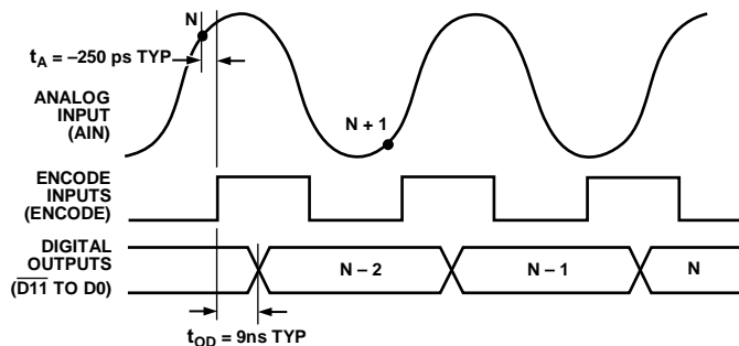
Figure 19. Timing Diagram
