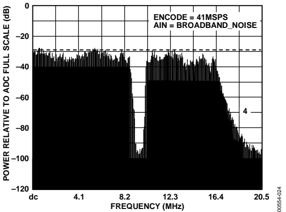
Figure 12. NPR Output Spectrum
