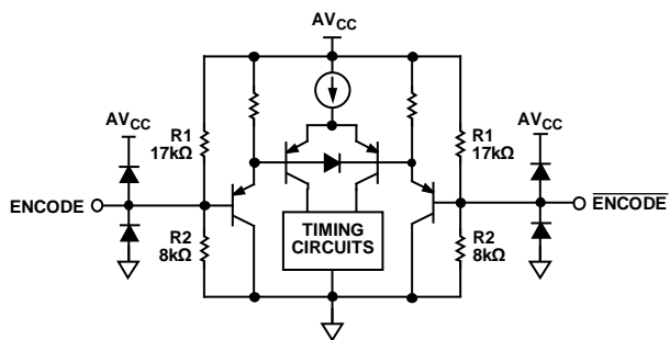
Figure 21. Encode Inputs
