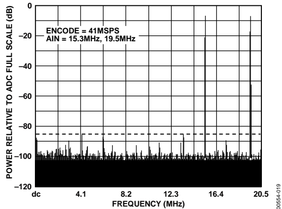
Figure 9. Two Tones at 15.3 MHz and 19.5 MHz
