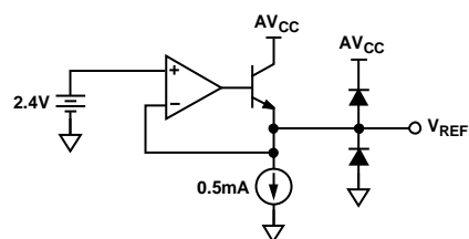
Figure 24. 2.4 V Reference
