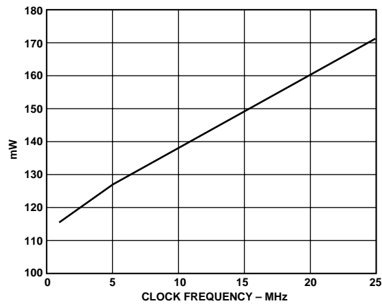
Figure 8. Power Consumption vs. Sample Rate
