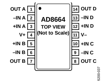
Figure 6. AD8664, 14-Lead TSSOP (RU-14)
