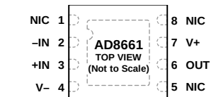
Figure 2. AD8661, 8-Lead LFCSP (CP-8-13)
