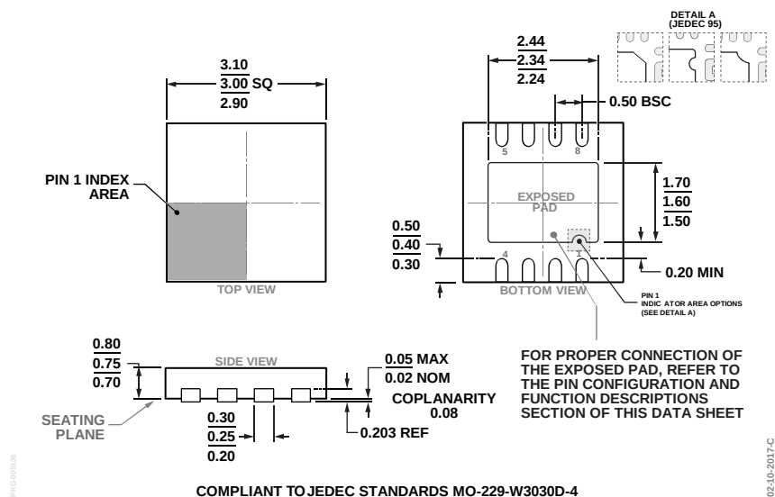
Figure 80. 8-Lead Lead Frame Chip Scale Package [LFCSPP] 3 mm x 3 mm Body and 0.75 mm Package Height (CP-8-11)
