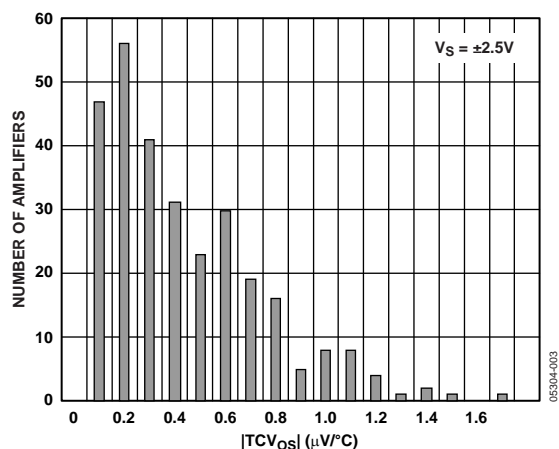
Figure 5. |TCV_{OS}| Distribution
