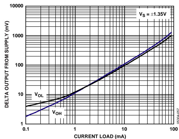
Figure 36. AD8656 Output Swing vs. Current Load
