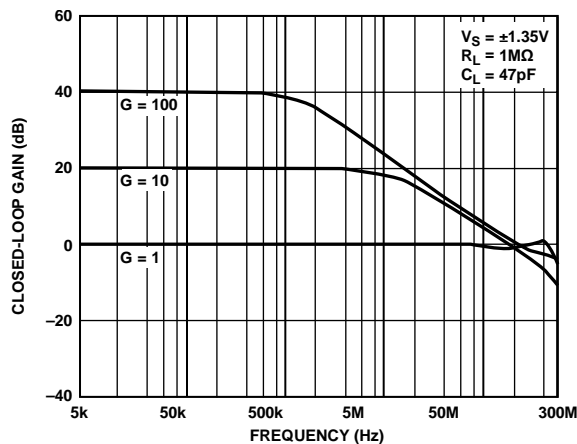
Figure 51. Closed-Loop Gain vs. Frequency
