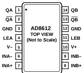
Figure 3. 14-Lead TSSOP (RU-14)
