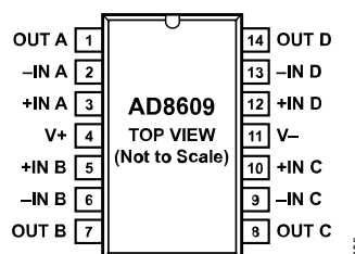
Figure 5. 14-Lead SOIC (R Suffix)
