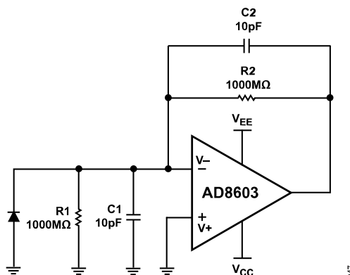
Figure 47. Photodiode Circuit
