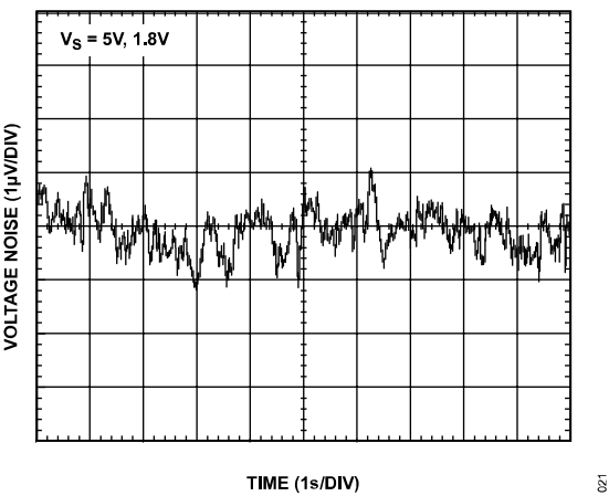
Figure 21. 0.1 Hz to 10 Hz Input Voltage Noise
