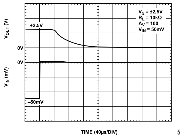
Figure 24. Negative Overload Recovery
