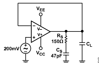
Figure 43. Snubber Network
