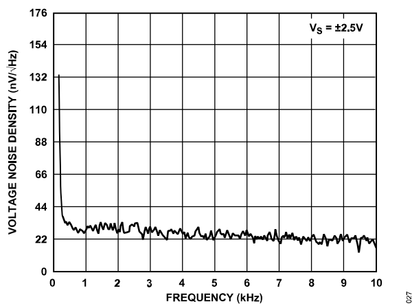
Figure 27. Voltage Noise Density vs. Frequency
