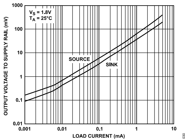
Figure 30. Output Voltage to Supply Rail vs. Load Current
