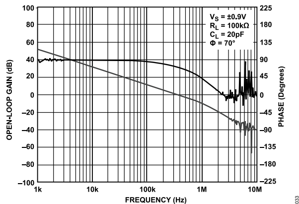
Figure 33. Open-Loop Gain and Phase vs. Frequency
