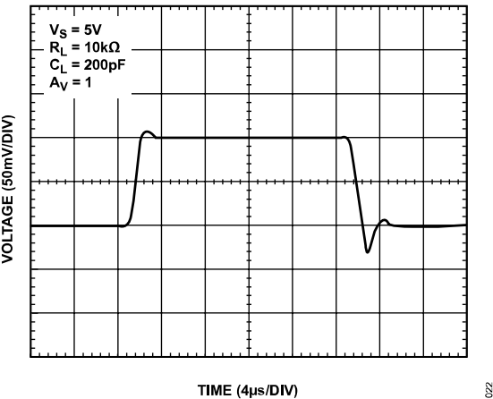
Figure 22. Small Signal Transient
