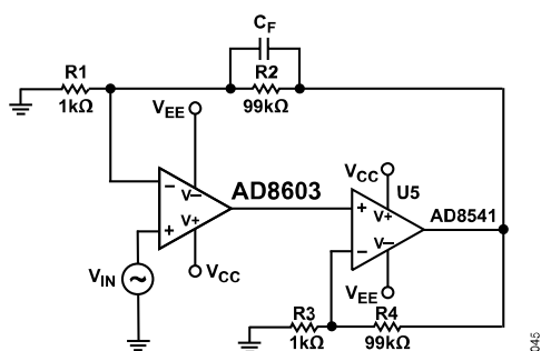
Figure 45. High Gain Composite Amplifier
