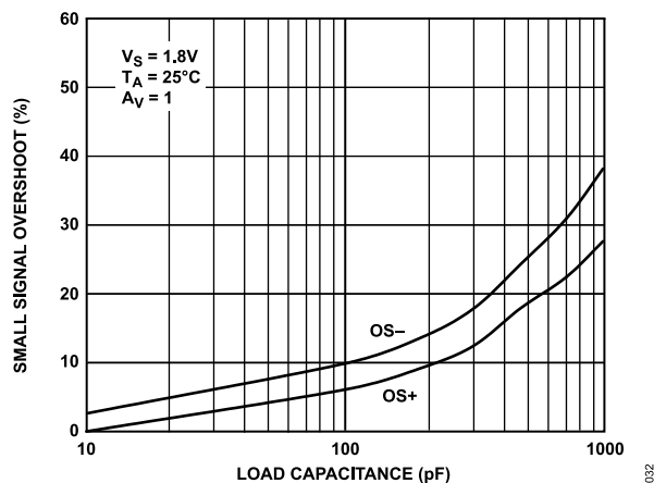
Figure 32. Small Signal Overshoot vs. Load Capacitance
