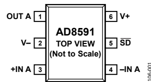
Figure 1. 6-Lead SOT-23 (RJ Suffix)
