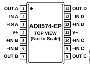
Figure 1. 14-Lead TSSOP
