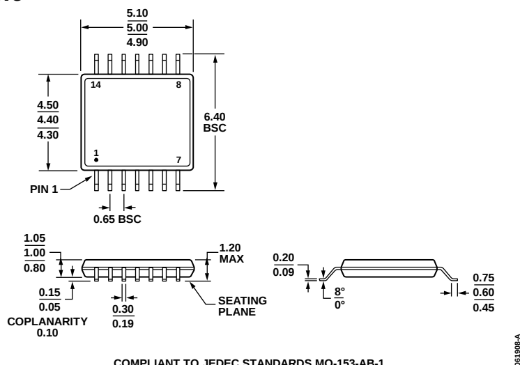
Figure 45. 14-Lead Thin Shrink Small Outline Package [TSSOP] (RU-14)
