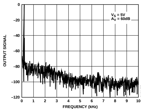
Figure 58. Spectral Analysis of AD8572 in High Gain with an Input Signal
