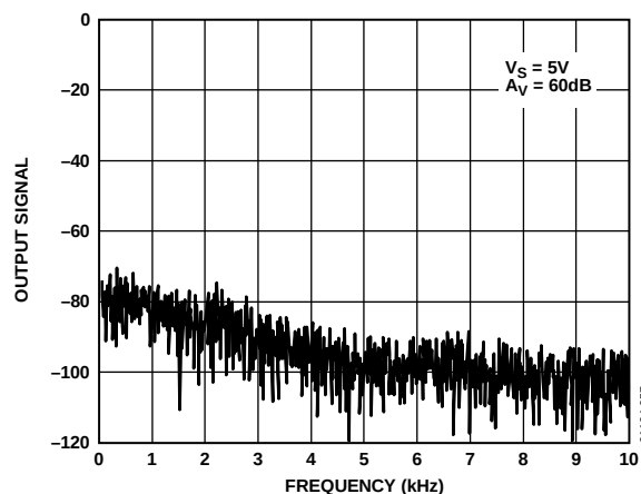
Figure 57. Spectral Analysis of AD8571/AD8572/AD8574 Output with 60 dB Gain
