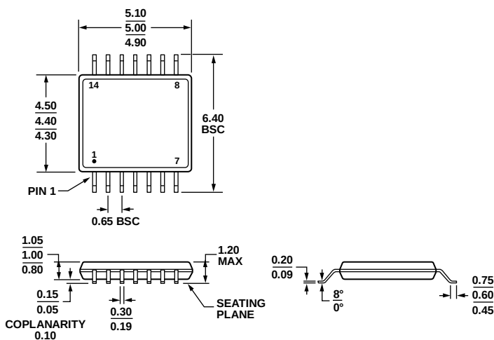
Figure 72. 14-Lead Thin Shrink Small Outline Package [TSSOP] (RU-14)
