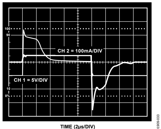
Figure 33. Scope Photo of the V_{\text{COM}} Instantaneous Peak Current
