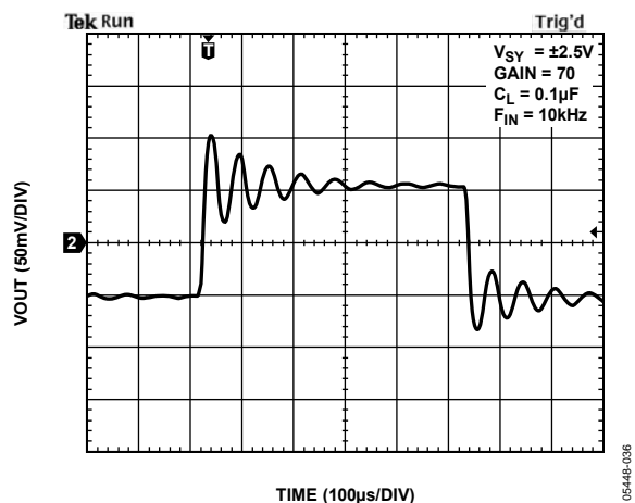
Figure 35. Small Signal Response at C_L = 0.1 \text{ µF} and F_{IN} = 10 \text{ kHz}
