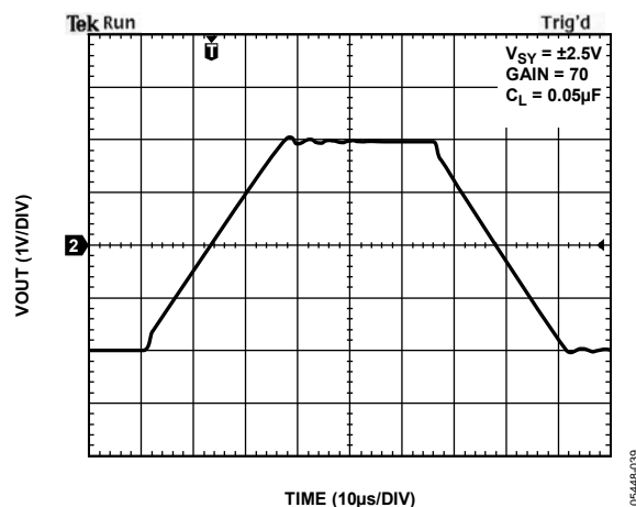
Figure 38. Large Signal Response at C_L = 0.05 \text{ µF}
