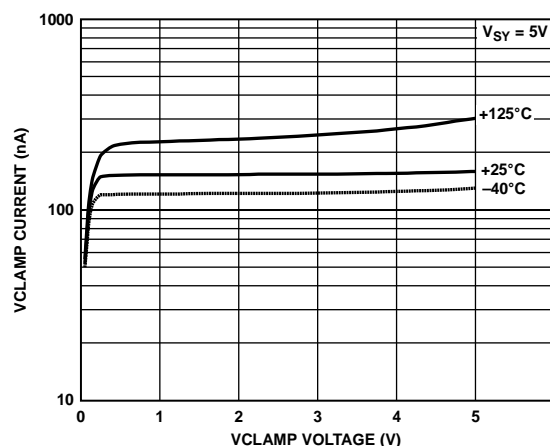
Figure 13. VCLAMP Current over Temperature at V_S = 5 V vs. VCLAMP Voltage
