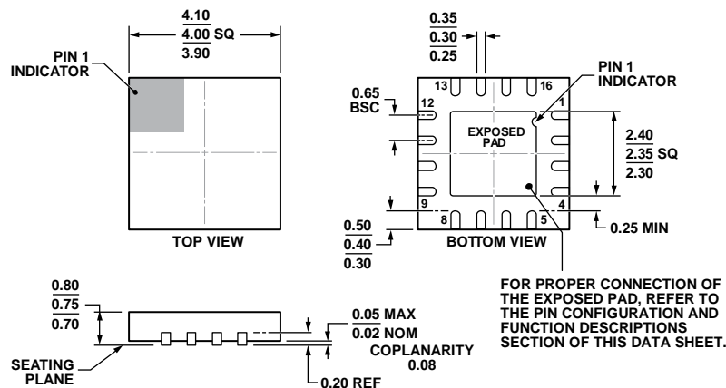
Figure 57. 16-Lead Lead Frame Chip Scale Package [LFCSP_WQ] 4 mm x 4 mm Body, Very Very Thin Quad (CP-16-20)
