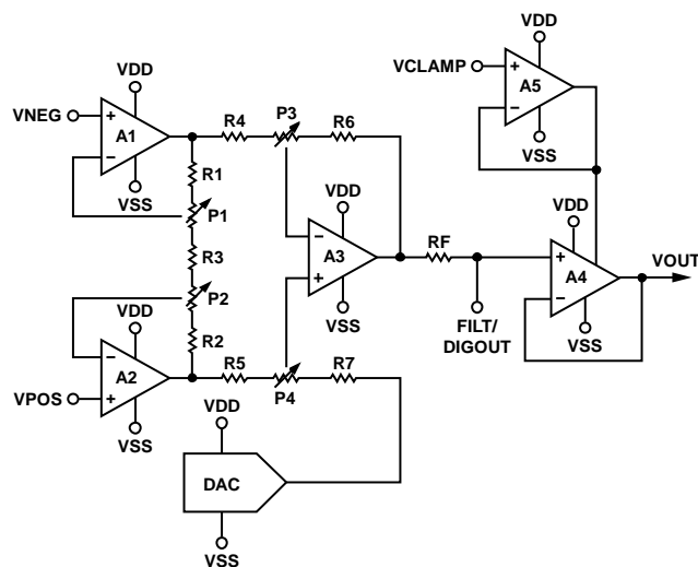
Figure 47. Functional Schematic
