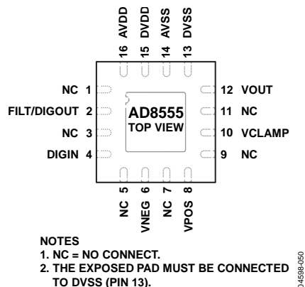
Figure 3. 16-Lead LFCSP (Not Drawn to Scale)
