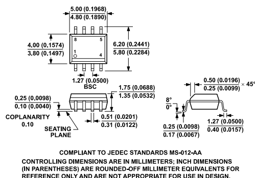
Figure 47. 8-Lead Standard Small Outline Package [SOIC_N] Narrow Body (R-8) Dimensions shown in millimeters and (inches)
