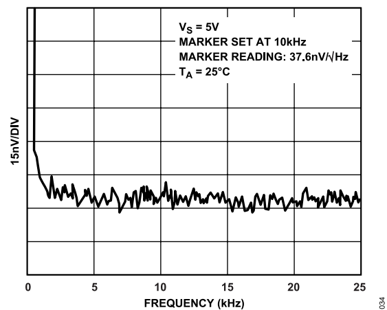
Figure 35. Voltage Noise
