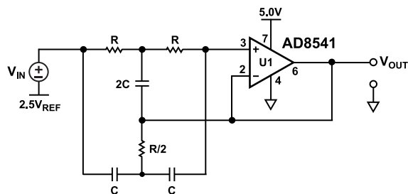
Figure 37. 60 Hz Twin-T Notch Filter, Q = ∞ (Ideal)
