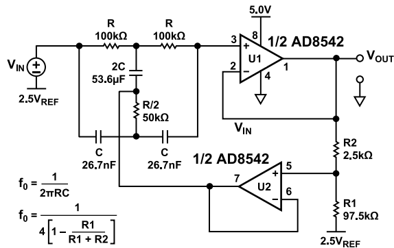
Figure 36. 60 Hz Twin-T Notch Filter, Q = 10
