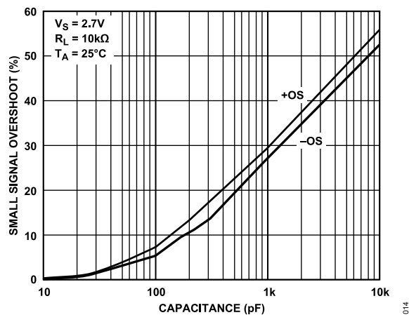
Figure 14. Small Signal Overshoot vs. Load Capacitance
