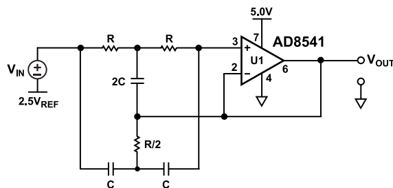
Figure 37. 60 Hz Twin-T Notch Filter, Q = ∞ (Ideal)
