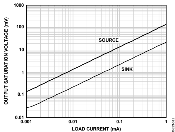
Figure 12. Output Saturation Voltage vs. Load Current, V_S = 5 V
