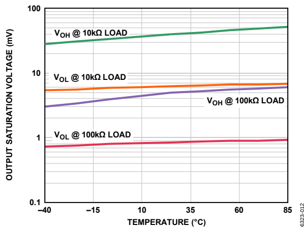
Figure 13. Output Saturation Voltage vs. Temperature, V_S = 5 V
