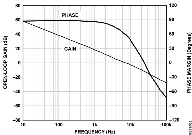
Figure 14. Open-Loop Gain and Phase vs. Frequency, V_S = 5 V
