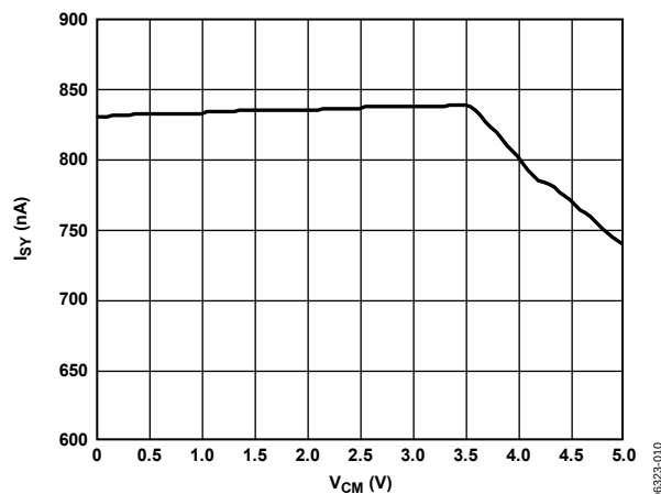
Figure 11. Supply Current vs. Input Common-Mode Voltage, V_S = 5 V
