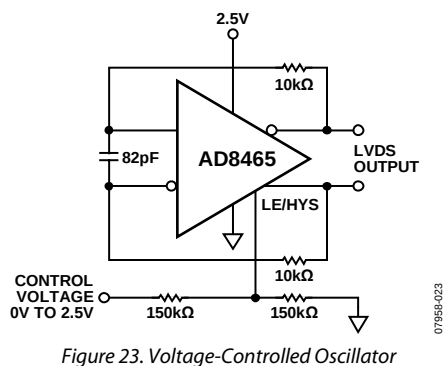
Figure 23. Voltage-Controlled Oscillator
