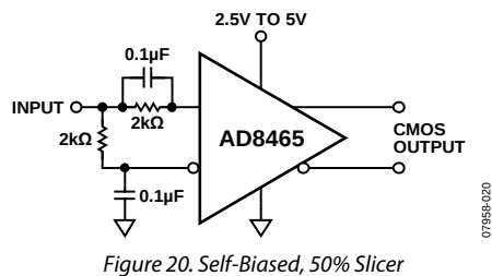
Figure 20. Self-Biased, 50% Slicer
