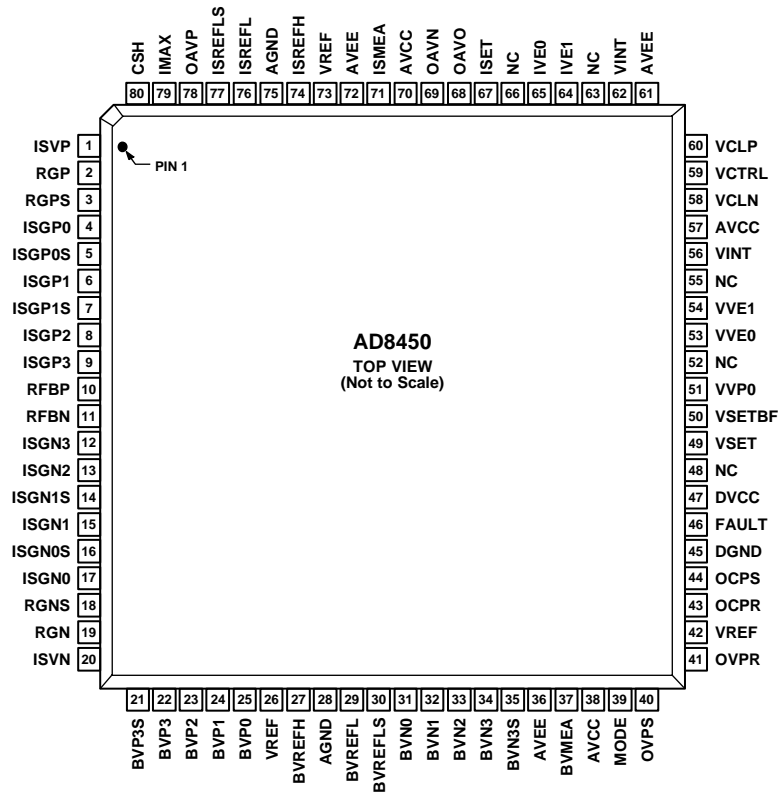
Figure 2. Pin Configuration
