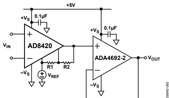
Figure 67. Output Buffering
