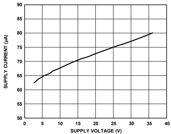
Figure 56. Supply Current vs. Total Supply Voltage
