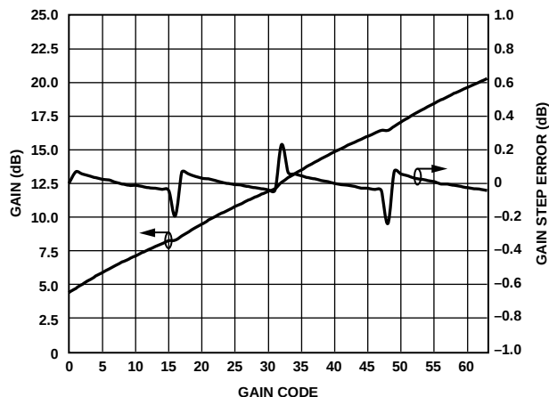
Figure 49. Gain and Gain Step Error vs. Gain Code at 10 MHz
