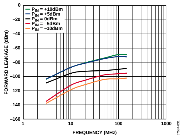
Figure 40. Forward Leakage vs. Frequency, Part Disabled
