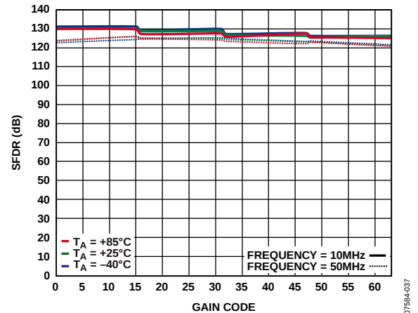
Figure 38. SFDR vs. Gain Code at 10 MHz and 50 MHz, 1 Hz Analysis Bandwidth
