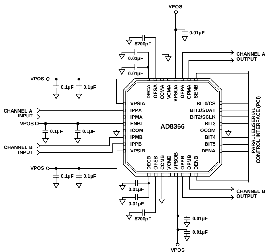
Figure 50. Basic Connections
