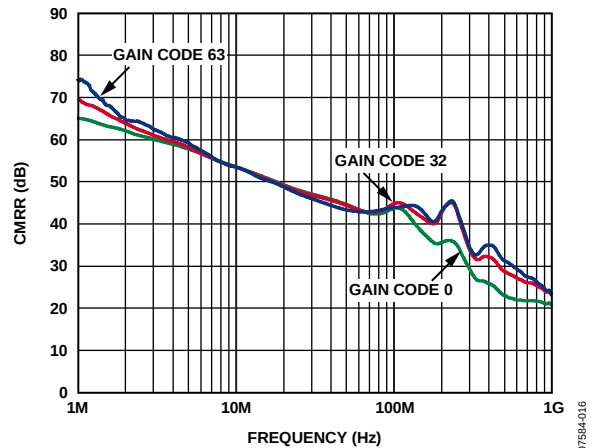
Figure 39. Common-Mode Rejection Ratio (CMRR) vs. Frequency
