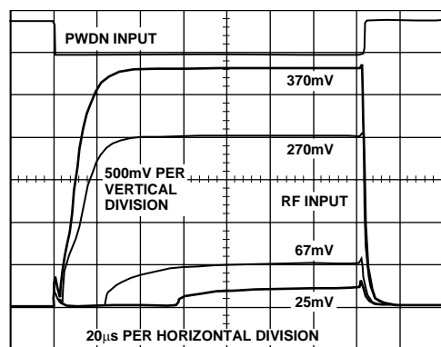
Figure 28. Output Response Using Power-Down Mode for Various RF Input Levels, Supply 3 V, Frequency 900 MHz, 0.01 \mu F Filter Capacitor
