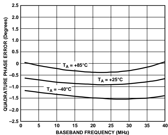
Figure 28. Quadrature Phase Error vs. F_{BB} , V_{GIN} = 0.7 V, V_S = 5 V
