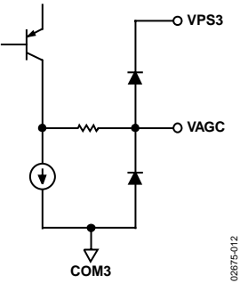
Figure 44. Circuit I
