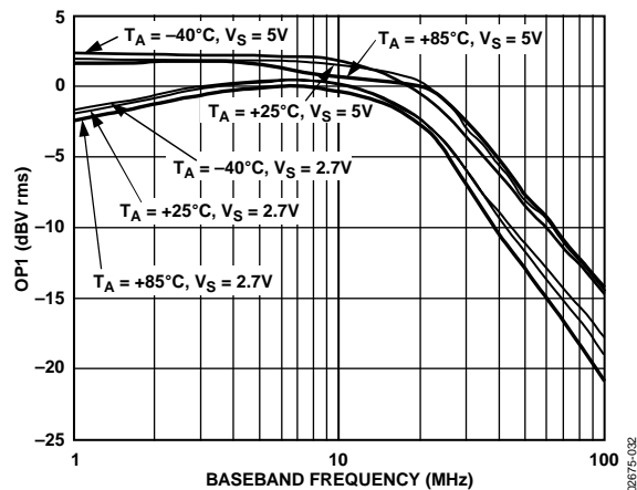
Figure 23. OP1 vs. F_{BB} , V_{CMO} = 1\text{ V}
