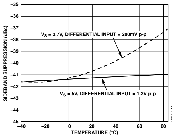
Figure 13. Sideband Suppression vs. Temperature ( F_{LO} = 800\text{ MHz} , LO Level = -2 dBm, F_{BB} = 1\text{ MHz} , I and Q Inputs Driven in Quadrature)
