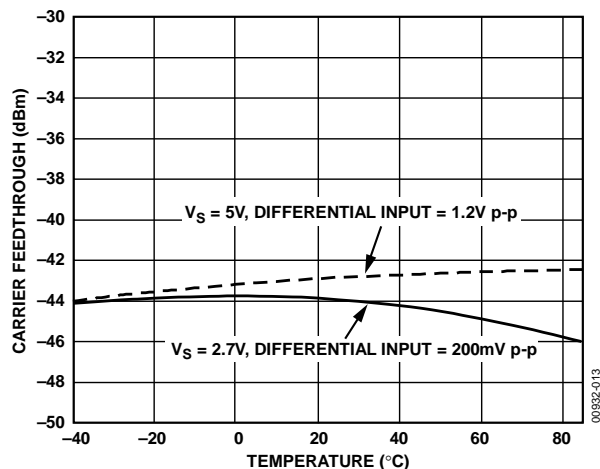
Figure 9. Carrier Feedthrough vs. Temperature ( F_{LO} = 800\text{ MHz} , LO Level = -2 dBm)
