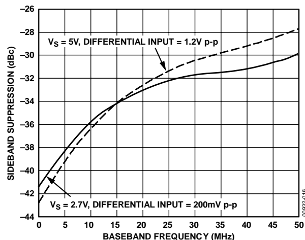
Figure 12. Sideband Suppression vs. F_{BB} ( T_A = 25^{\circ}\text{C} , F_{LO} = 800\text{ MHz} , LO Level = -2 dBm, I and Q Inputs Driven in Quadrature)
