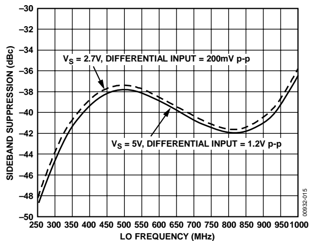
Figure 11. Sideband Suppression vs. F_{LO} ( T_A = 25^{\circ}\text{C} , LO Level = -2 dBm, F_{BB} = 1\text{ MHz} , I and Q Inputs Driven in Quadrature)
