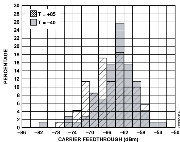
Figure 10. Carrier Feedthrough Distribution at Temperature Extremes After Feedthrough Nulled to < -65\text{ dBm} at T_A = 25^{\circ}\text{C} ( F_{LO} = 800\text{ MHz} , LO Level = -2 dBm)
