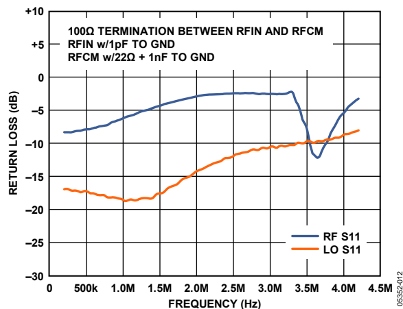
Figure 58. RF and LO Return Loss with Matching
