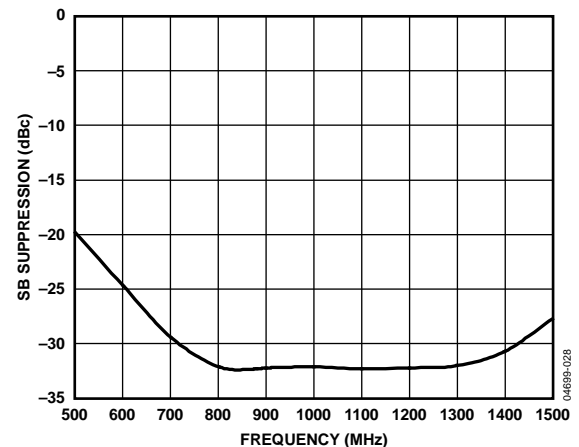
Figure 28. Sideband Suppression vs. Frequency
