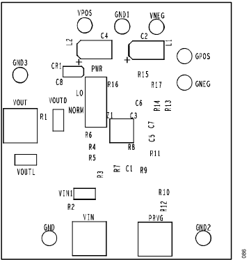
Figure 84. Secondary Side Copper
