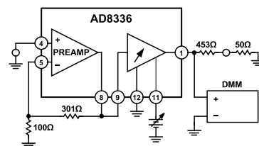
Figure 60. Offset Voltage
