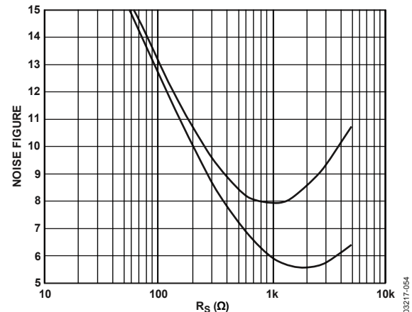
Figure 53. Noise Figure for Source Resistance of 50 \Omega to 5 k \Omega , at f = 10 MHz (Lower) and 100 MHz (Simulation)
