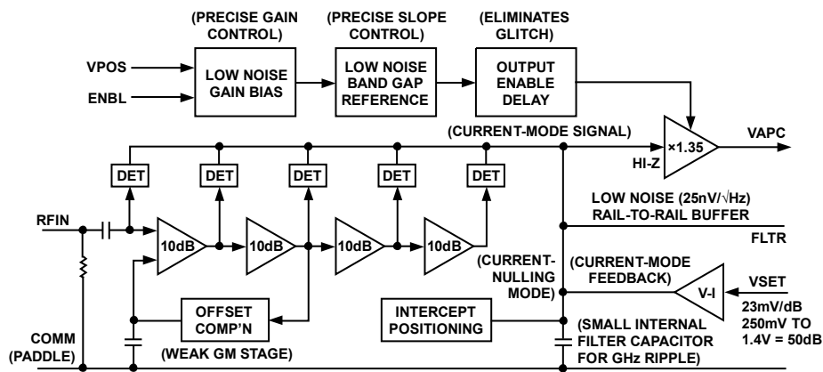
Figure 32. Block Schematic
