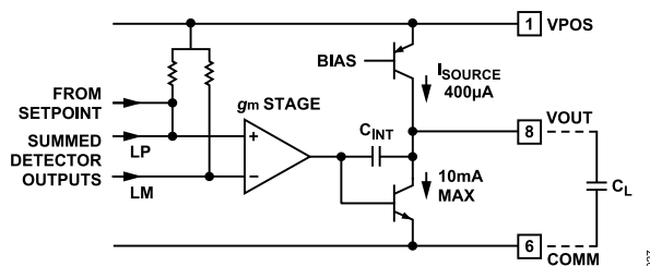
Figure 27. Output Interface Circuitry
