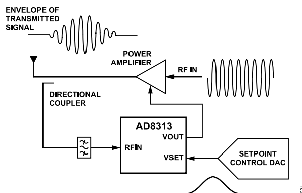
Figure 31. Setpoint Controller Operation
