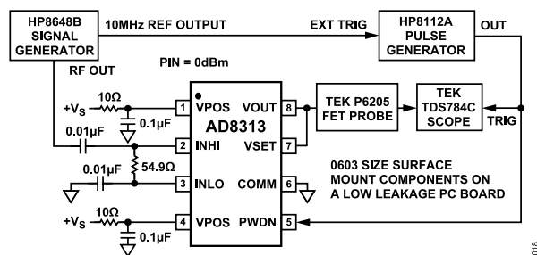
Figure 18. Test Setup for PWDN Response Time
