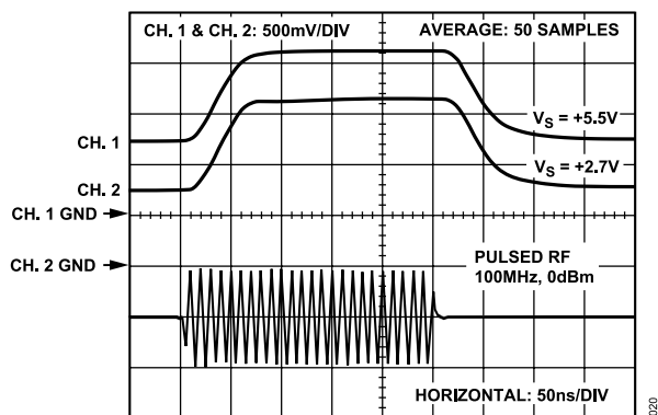
Figure 20. Response Time, No Signal to 0 dBm
