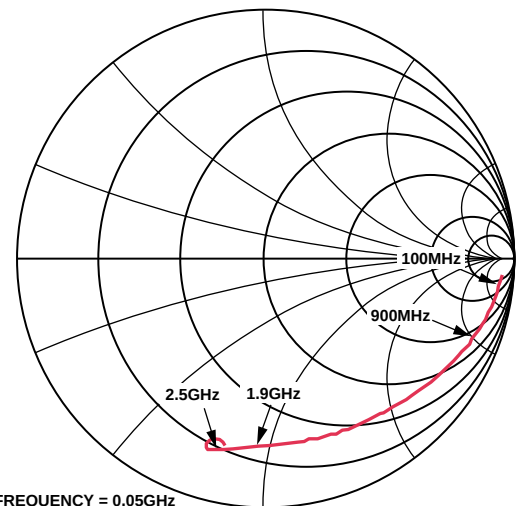
START FREQUENCY = 0.05GHz STOP FREQUENCY = 3.5GHz
