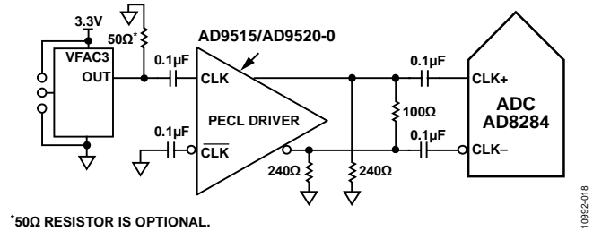
Figure 18. Differential PECL Sample Clock
