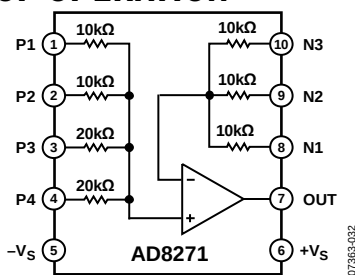
Figure 43. Functional Block Diagram
