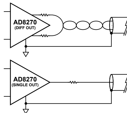
Figure 50. Driving Cabling
