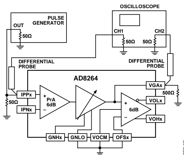
Figure 99. Pulse Response to V_{GAX} , V_{GAIN} = 0.7\text{ V} (See Figure 55 and Figure 57)
