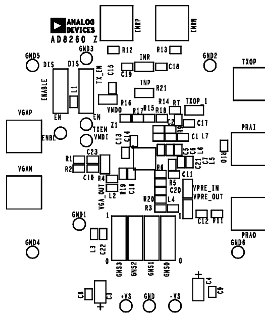
Figure 76. AD8260-EVALZ Component Side Silkscreen
