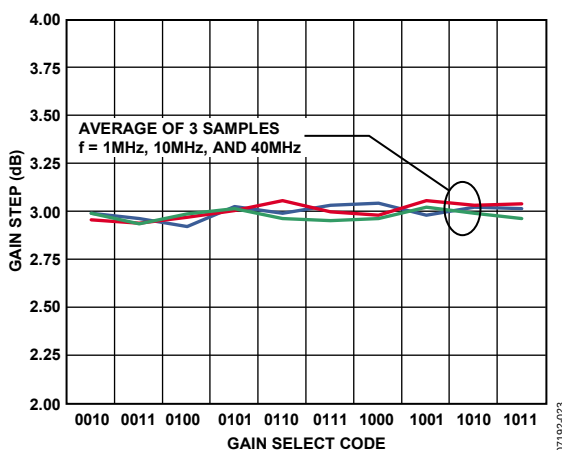
Figure 23. Gain Step vs. Gain Select Code for Three Samples for the VGA/Preamplifier at Three Frequencies—See Figure 57
