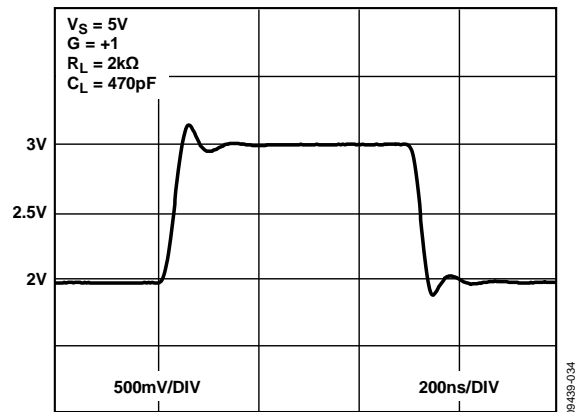
Figure 36. Pulse Response, +V_S = +5\text{ V} , G = +1 , C_L = 470\text{ pF}
