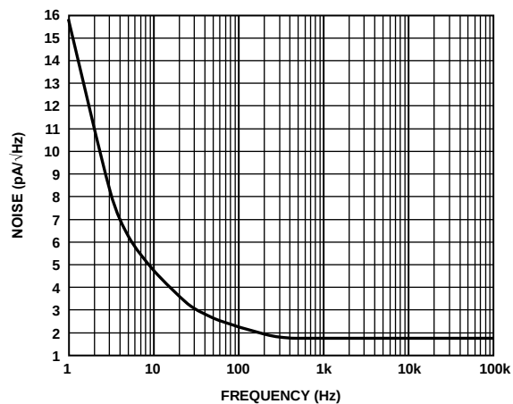
Figure 40. Current Noise Spectral Density vs. Frequency
